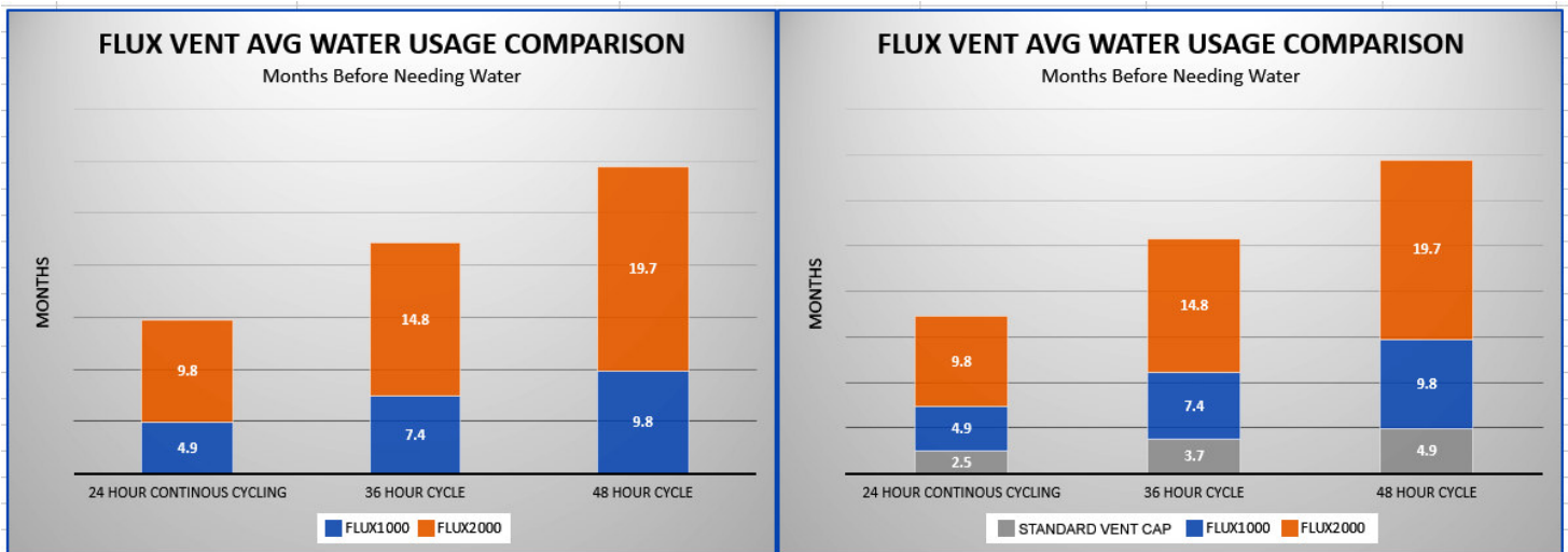
Battery Recombination Caps Water Savings Chart
